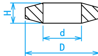
SECTION VIEW
